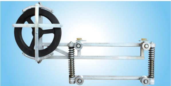
新电缆小车 New cable trolley 安装方便,安装吊笼下方导轨或对面导轨上,与吊笼运行轨道相同,受风力影响较小,独特的机构设计,可有效降低进出门槛高度,减少施工量。 Installed easily, it is installed on the mast under the cage or on the opposite mast and same track with the cage running not affected by the wind, it is with special construction design, so that reduce the threshold and the construction.
