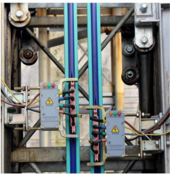
滑触线 Sliding contact line 拔插式新型滑触线,具有安装方便,不受风载影响,压降低,低进出门槛的特点。 Pull and plug type sliding contact line has the features: easy installation,not effected by the wind, low pressure drop, and low sil.
