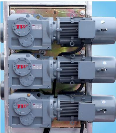
TW斜伞齿轮三传动 TW bevel gear three-motor.
