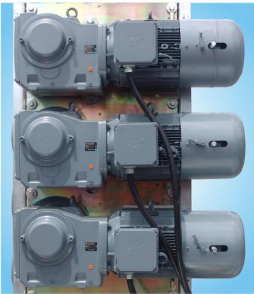
进口电机三传动 Three-motor for imported drive.
