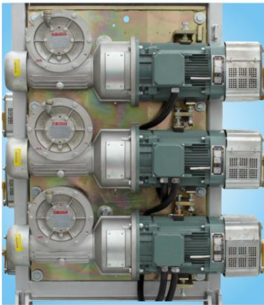
国产电机三传动 Three-motor for domestic drive.
